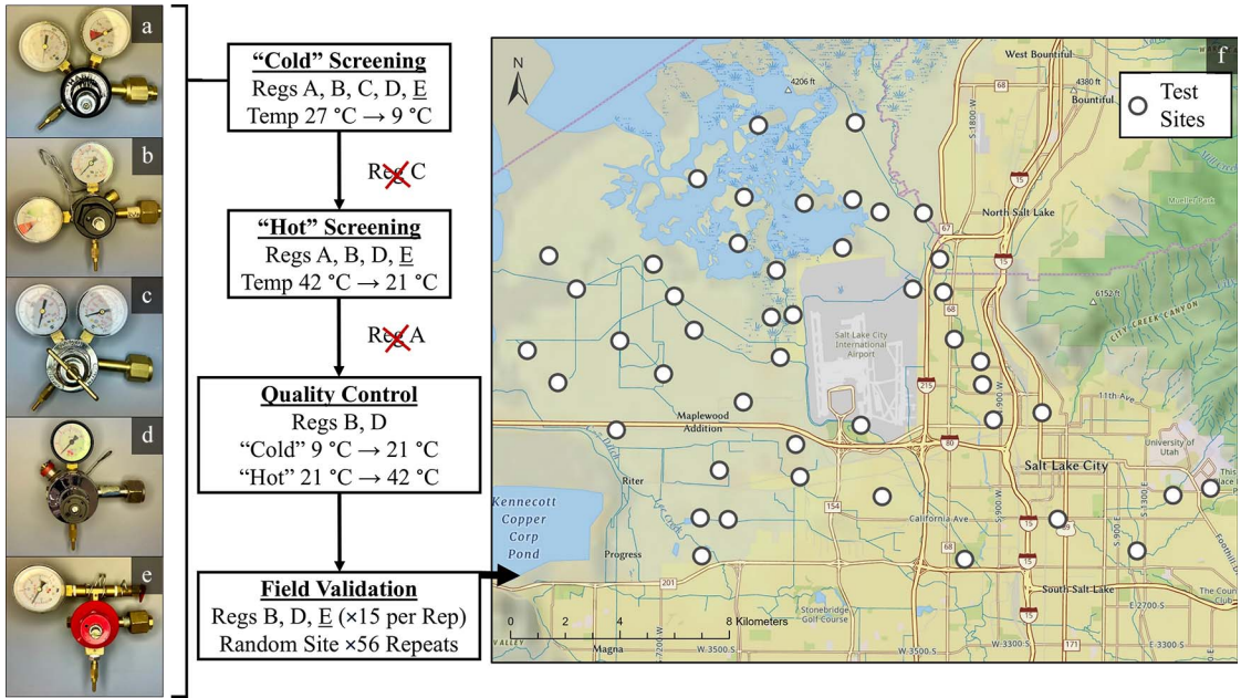
Fig. 1. Single-stage regulators were acquired from beverage and welding supply manufacturers (a-d) and compared to the preexisting, mass-used regulators (e) within the Salt Lake City Mosquito Abatement District for use with pressurized gas cylinders dispensing CO 2 . Tolerance tests were conducted using environmental chambers to screen for cold temperature failures, followed by rejection of models that failed. Remaining models were screened again with hot temperature tests, followed by a second round of rejections for failed models. Remaining models were used in quality control tests with duplicates of regulators maintaining calibrations in prior stress tests. Final candidate regulators were deployed alongside the preexisting standard (Regulator E) in sets of 15 for a span of 52 trap nights across the SLCMAD surveillance network (f).
