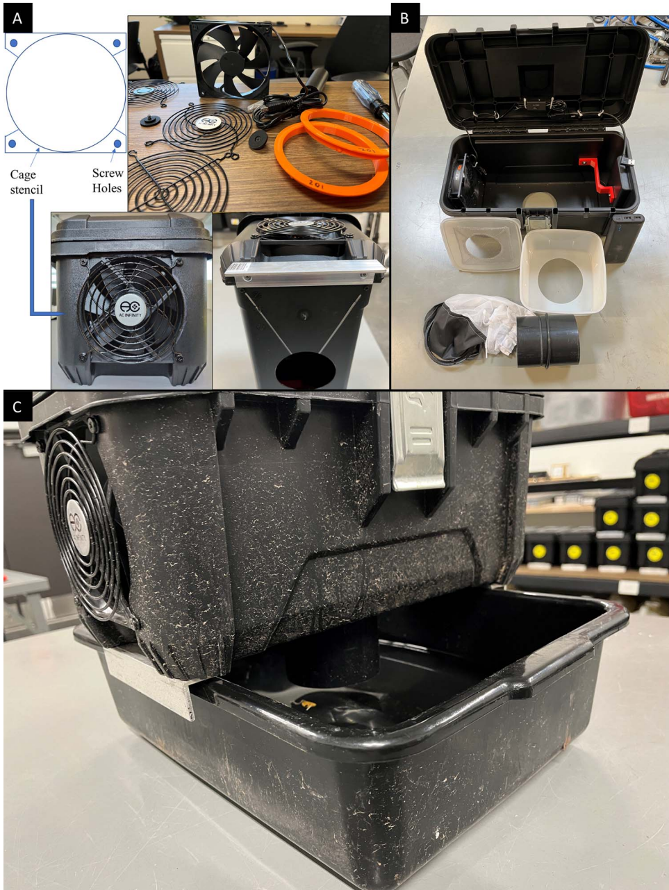
Fig. 1. Parts layout (A) and basic assembly (B) for the Salt Lake gravid trap (SLGT) version of the traditional Reiter-Cummings gravid trap. A computer case fan was used to stencil a pattern on a basic toolbox. Holes were cut such that the fan case pieces could screw directly through the plastic of the toolbox. Additional portholes and brackets were added to allow insert f cables, battery, collection container, and associated funnel pieces for the completed trap. The deployment procedure is identical to prior Reiter-Cummings style traps (C).
