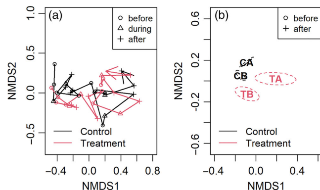
FIGURE 3 Nonmetric multidimensional scale (NMDS) ordination of insect diversity and composition at control and treatment sites. NMDS plot is based on Bray–Curtis similarity matrix using \log_{10}(x + 1) transformed insect family data. Points closer together had more similar insect diversity and composition. (a) Insect diversity and composition trajectory through time. Each point along the trajectory corresponds to a date classified as “before,” “during,” or “after” aerial application of insecticides. Arrow represents the end point. Stress = 0.065. (b) Insect diversity and composition by group (C—control; T—treatment) before (B) and after (A) the aerial application of insecticides. Dashed contours indicate confidence limits around each group defined by standard deviation of the points. Each point corresponds to an individual site within the group ( n = 3 for control, n = 7 for treatment). Stress = 0.064
